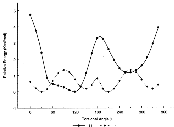
Figure 5. A comparison of potential energy curves (PEC) for the torsional angle \phi of compounds 4 and 11 each calculated from AM1 calculations.
